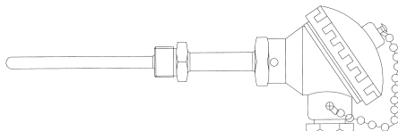
Fig 31: Industrial Probe with Flange and Lagging Extension
