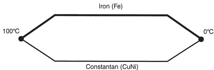
Fig 1: Thermoelement Circuit
