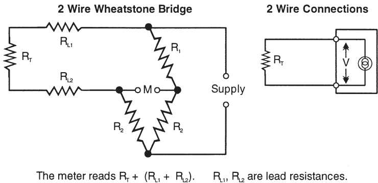
Fig 15: Practical Bridge Circuits for 2, 3 and 4 Wire Thermometers.
