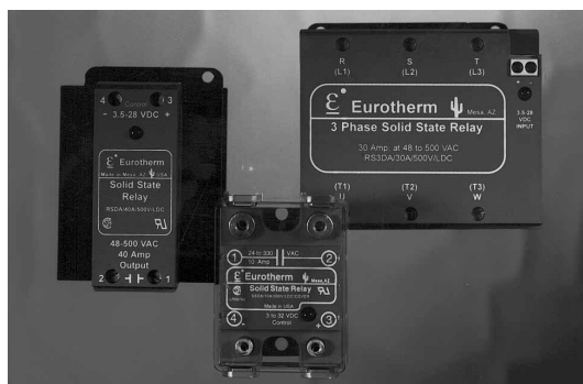
Fig 48: Solid State Power Switches for Electrical Heaters
