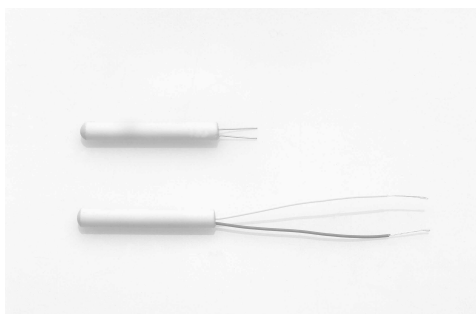
Fig 17: Pt100 Resistors
