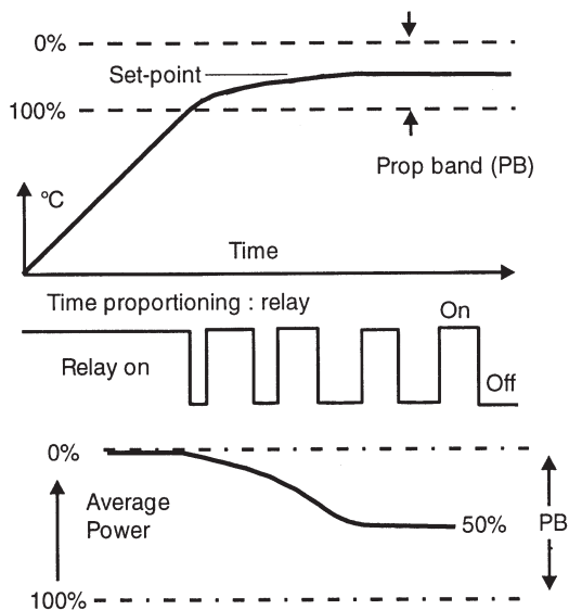
Fig 53: Proportional Control
